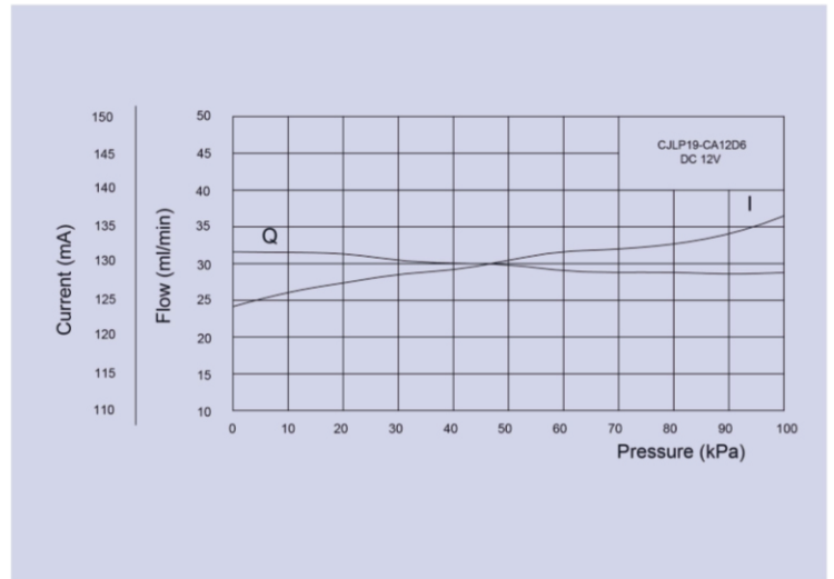
產品特性圖 Performance Curve
