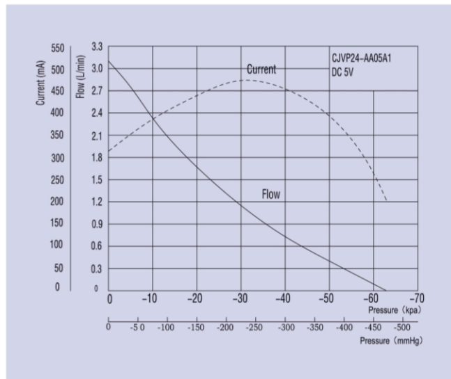
產品特性圖 Performance Curve
